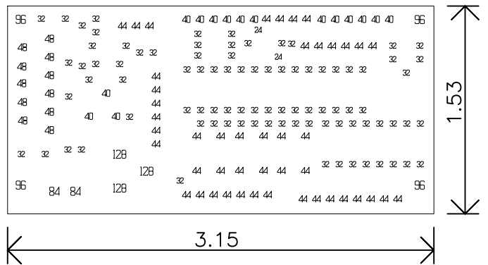
DRILL & OUTLINE
